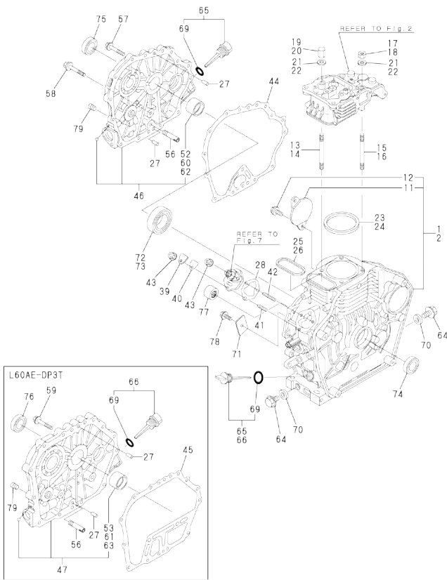
Fig.1. CYLINDER BLOCK
