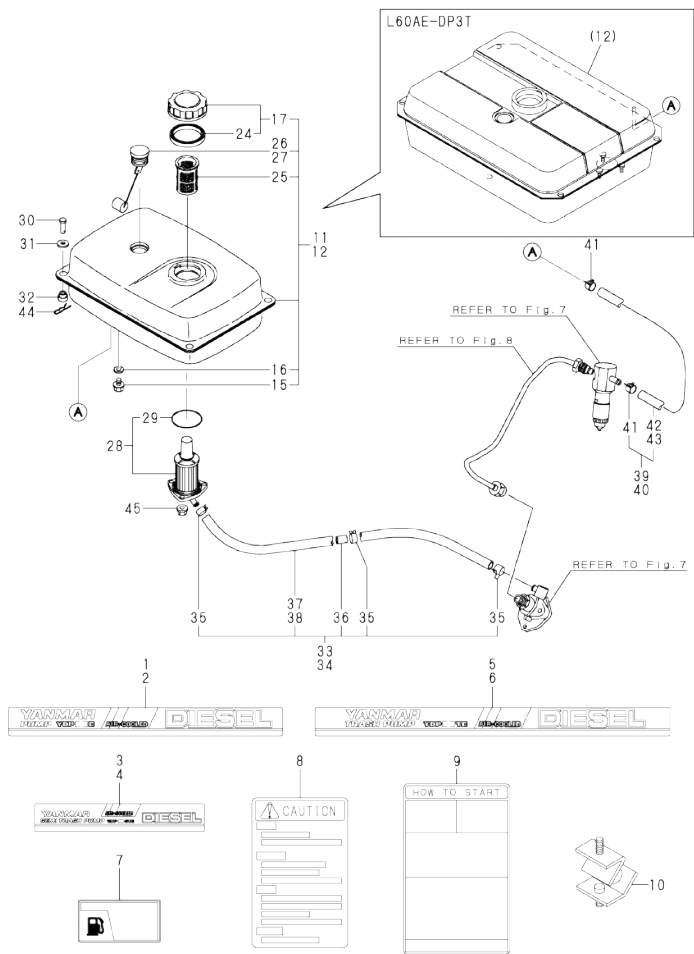
Fig.10. PACKAGED PART
