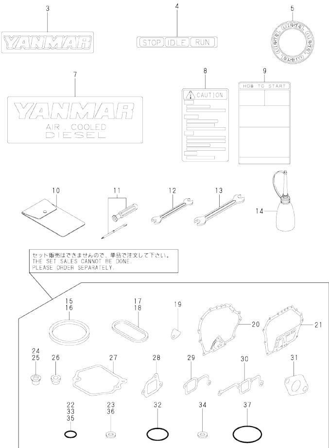
Fig.9. TOOL,LABEL & GASKET SET
