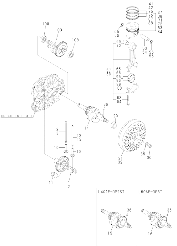
Fig.4. CRANKSHAFT,PISTON & CAMSHAFT
